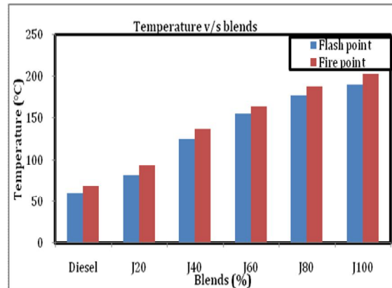
Fig.3.3 Temperature v/s Blends
