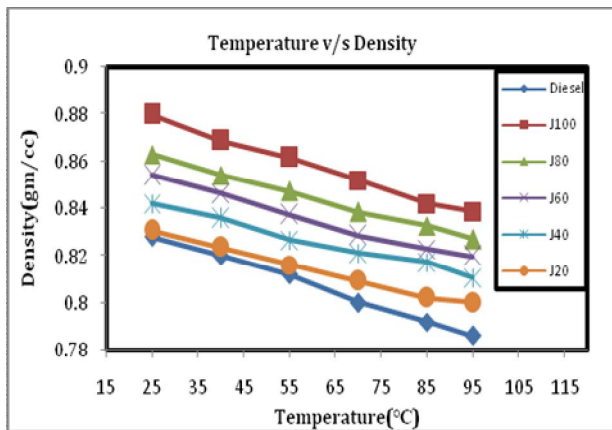
Fig.3.2 Density v/s Temperature
