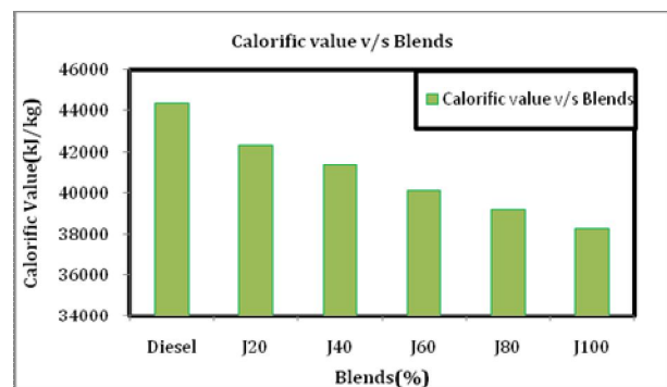
Fig.3.4 Calorific value v/s Blends
