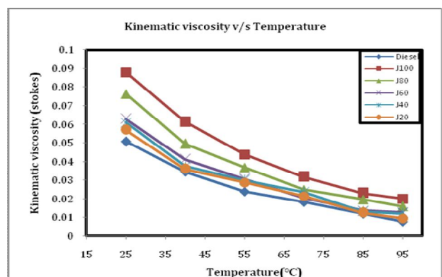
Fig 3.1 Kinematic viscosity v/s Temperature
