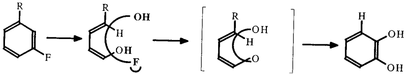
Figure 10. Possible mechanism of defluorination of 3-fluoro substituted benzenes by Pseudomonas sp, strain T-12 involving toluene-2,3-dioxygenase. Reprinted from Renganathan, App & Env Mic , vol. 55 #2, Feb. '89, p. 332.
