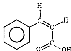
4 hydroxyperinaphthenone
