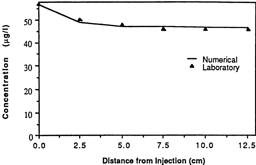
Figure 7. Numerical fit to the BF profile at a detention time of 125 min. The k and K_s are 0.013 \mu\text{g}/\text{mg cell-day} and 9.5 \mu\text{g}/\text{l} , respectively.
