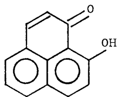
4 hydroxyperinaphthenone
