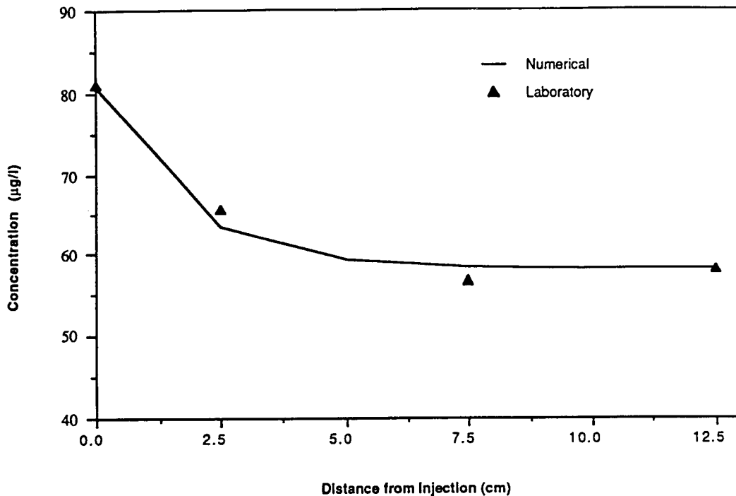
Figure 4. Numerical curve fit to the CTC profile at a detention time of 50.0 min. The k and K_s are 0.030 \mu\text{g}/\text{mg} cell-day and 4.5 \mu\text{g}/\text{l} , respectively.
