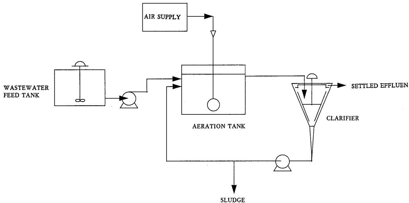
Figure 3. Schematic of a continuous-flow aeration unit.
