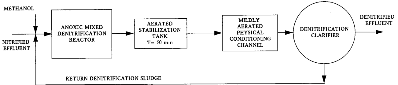
Figure 4. Suspended growth denitrification systems using methanol.
