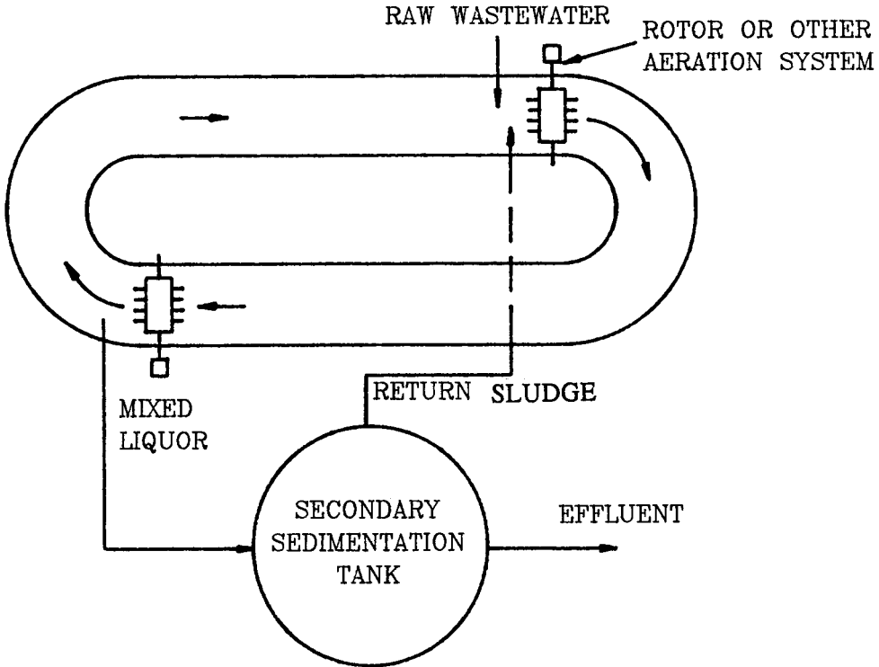
Figure 9. Pasveer ditch or endless channel system for nitrogen removal.
