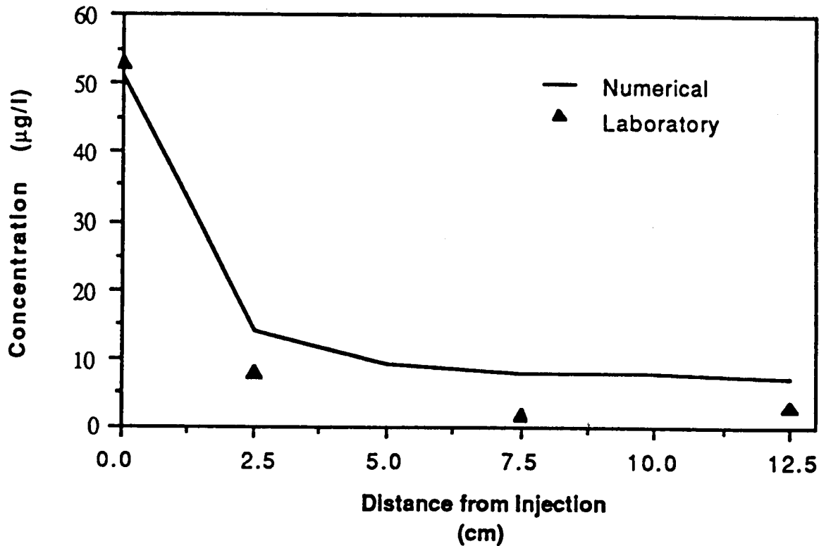
Figure 6. Prediction of the CTC profile at a detention time of 500 min. and with k = 0.030 \mu\text{g}/\text{mg cell-day} and K_s = 4.5 \mu\text{g}/\text{l} .
