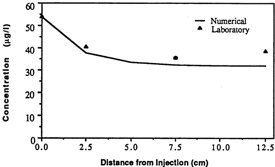
Figure 8. Prediction of the BF profile at a detention time of 500 min. and with k = 0.013 \mu\text{g}/\text{mg cell-day} and K_s = 9.5 \mu\text{g}/\text{l} .
