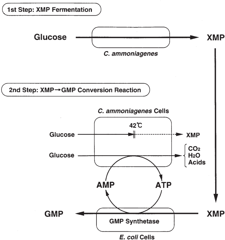
Fig. 2. Hybrid process to produce 5'-GMP catalyzed by cells of Corynebacterium ammoniagenes and recombinant E. coli
