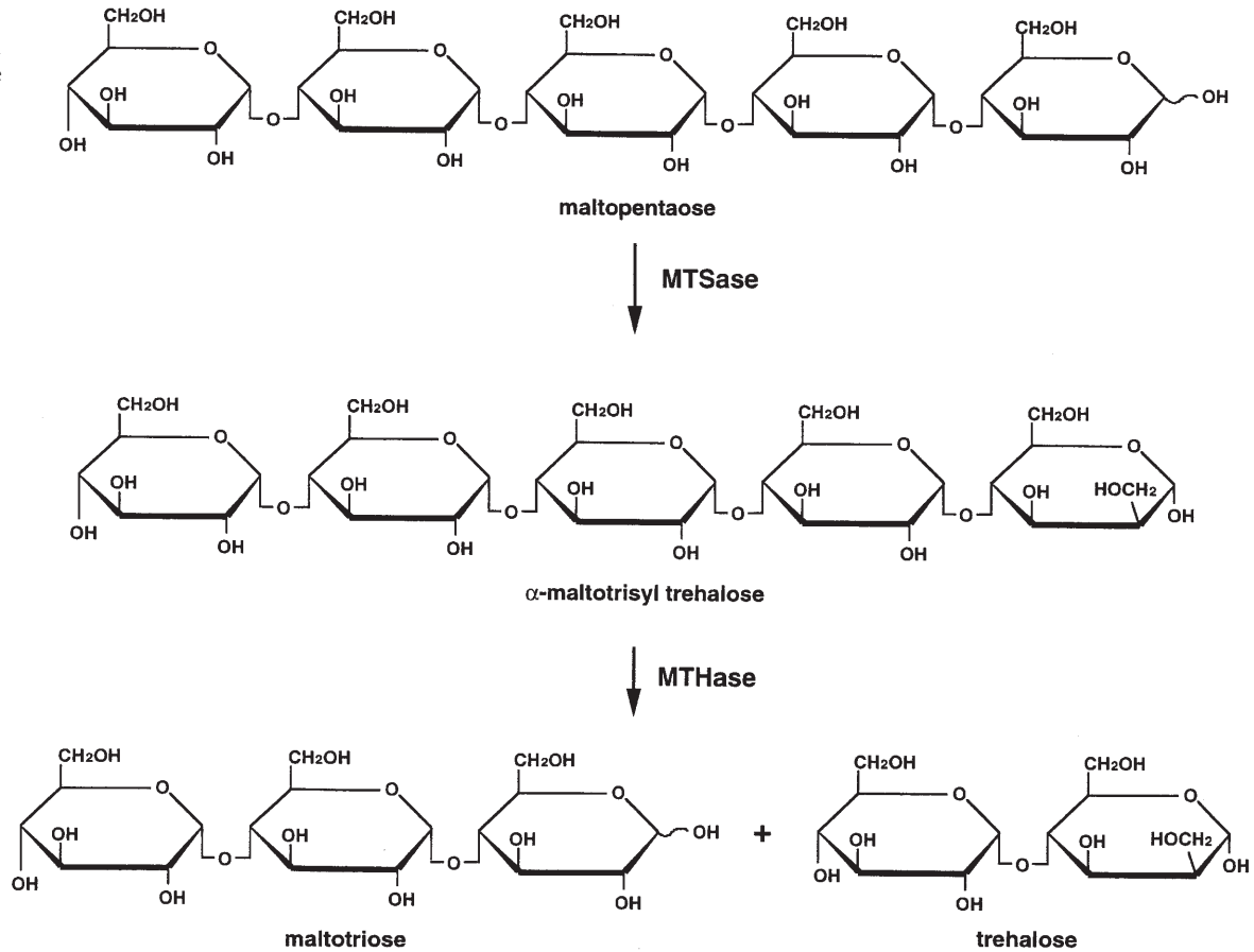
Fig. 5. Enzymatic system to produce trehalose from maltopentaose or amylose
