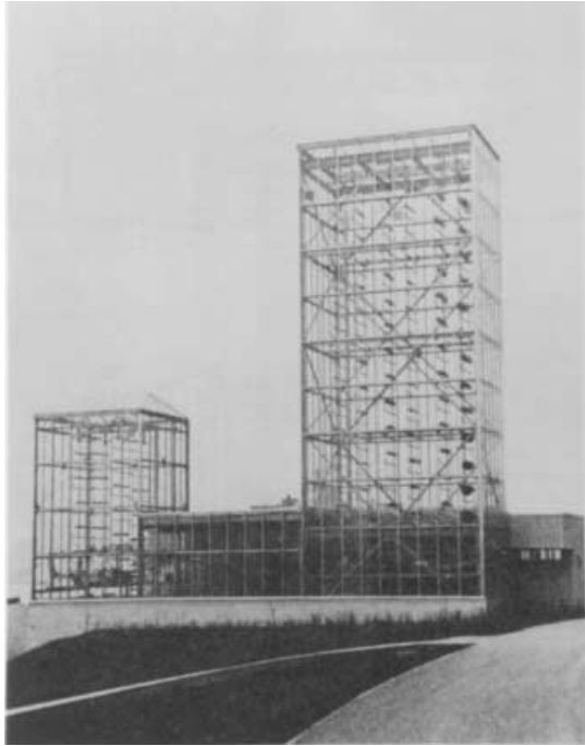
Fig. 3. Continuous industrial plant production system (O. Ruthner)
