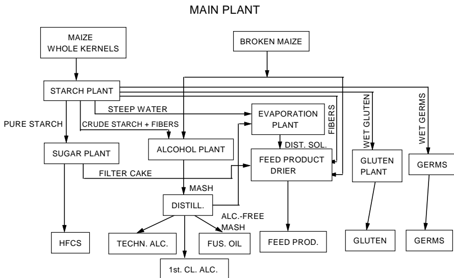
Fig. 3. General production scheme of the maize production complex in Szabadegyháza
