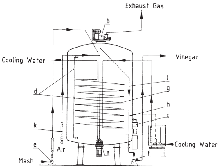
Fig. 5. Modern acetator for the production of vinegar (courtesy of Frings, Bonn)
