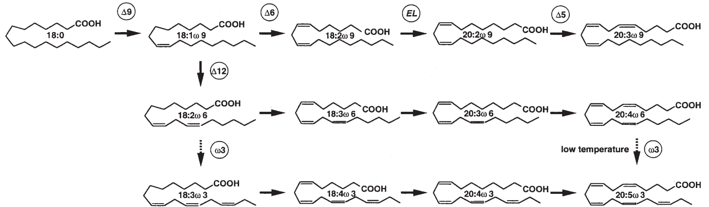
Fig. 3. Biosynthetic pathways of polyunsaturated fatty acids and the mutants of Mortiella alpina
