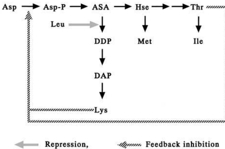
Fig. 1. Regulation of lysine biosynthesis. ASA, aspartate- \beta -semialdehyde; DDP, dihydrodipicolinate; DAP, \alpha , \epsilon -diaminopimelate; Hse, homoserine
